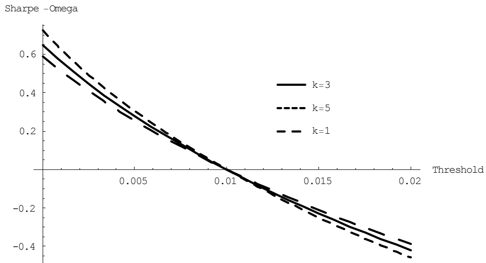
Exhibit 8 Sharpe-Omega Measure Various Levels of Monthly Kurtosis (Mean = 1%; Standard Deviation = 5%; Skewness = 0)
