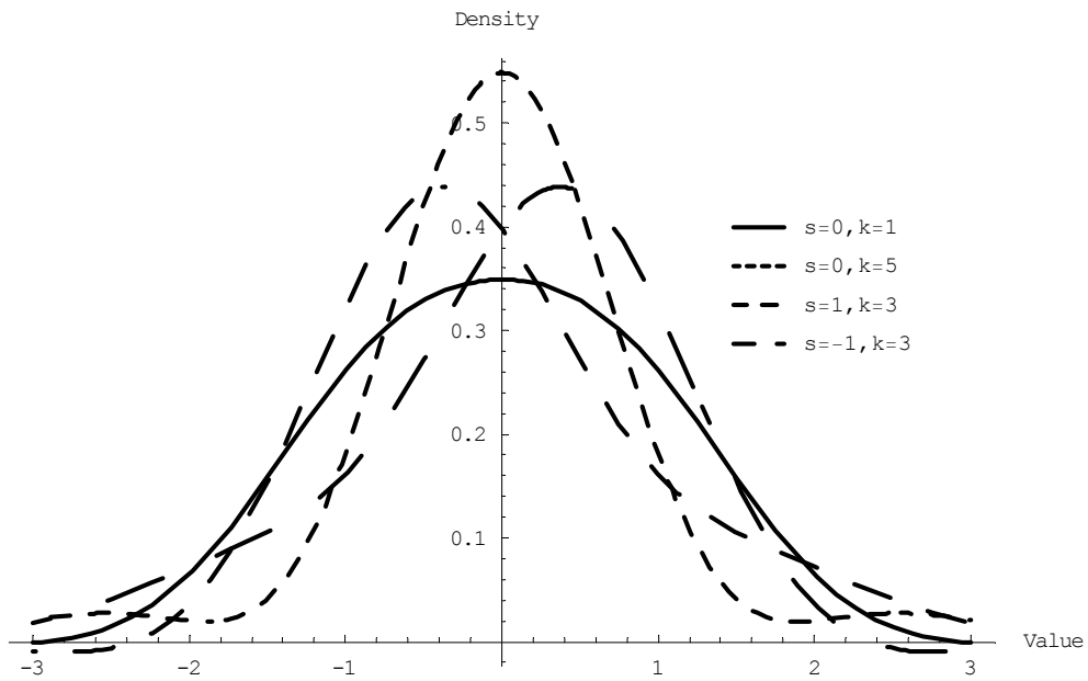
Exhibit 2 Density Function of the Four Parameter Johnson Distribution for Various Levels of Skewness and Kurtosis Mean = 0, Variance = 1
