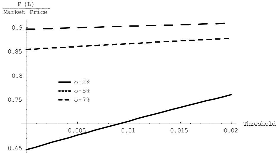
Exhibit 1 Ratio of P(L) to Market Put Prices for Various L and \sigma Monthly Figures Mean = 1%, Riskless Rate = 0.4%
