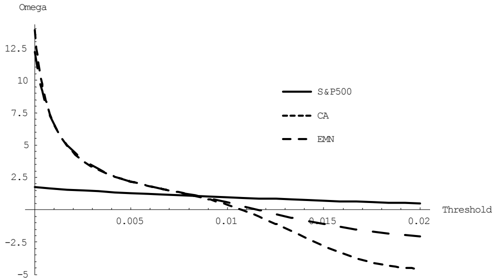
Exhibit 4 Omega Measure for S&P500, CSFB-Tremont Convertible Arbitrage and Equity Market Neutral Indices
