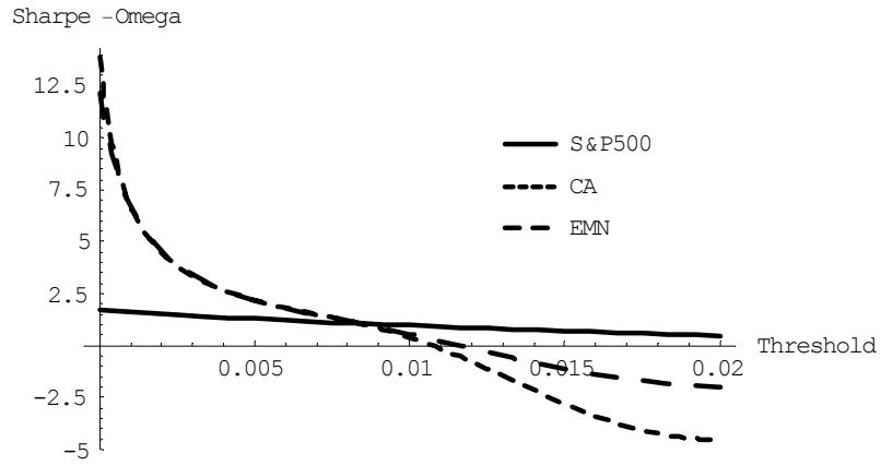
Exhibit 4 Omega Measure for S&P500, CSFB-Tremont Convertible Arbitrage and Equity Market Neutral Indices
