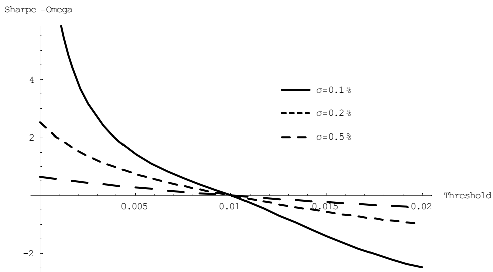
Exhibit 6 Sharpe-Omega Measure Various Levels of Monthly Standard Deviation (Mean = 1%; Skewness = 0; Kurtosis = 3)
